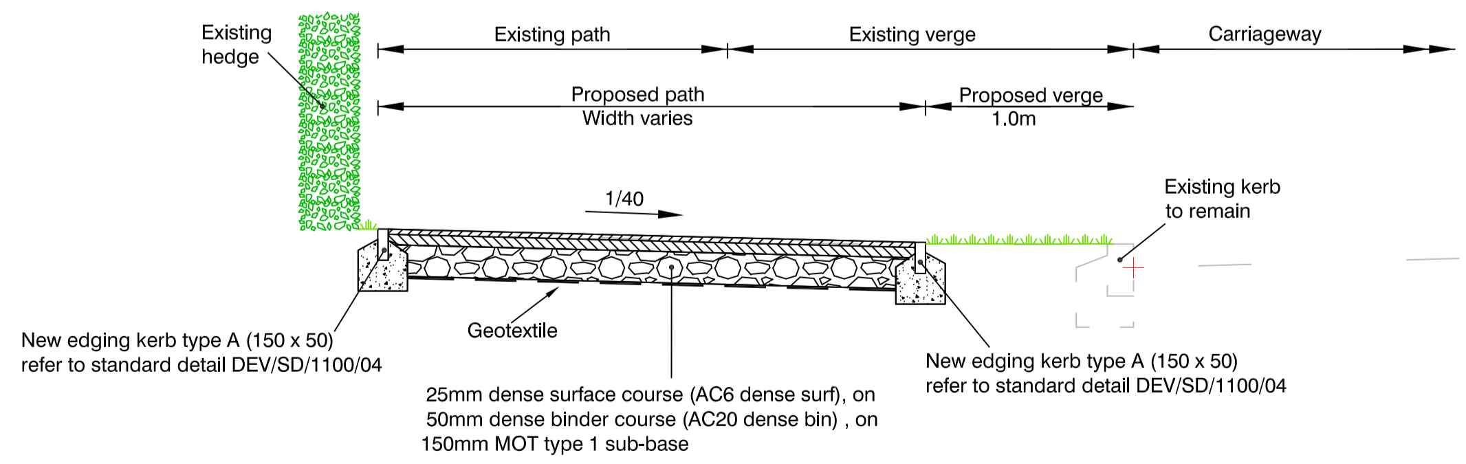
TYPICAL SECTION A-A
